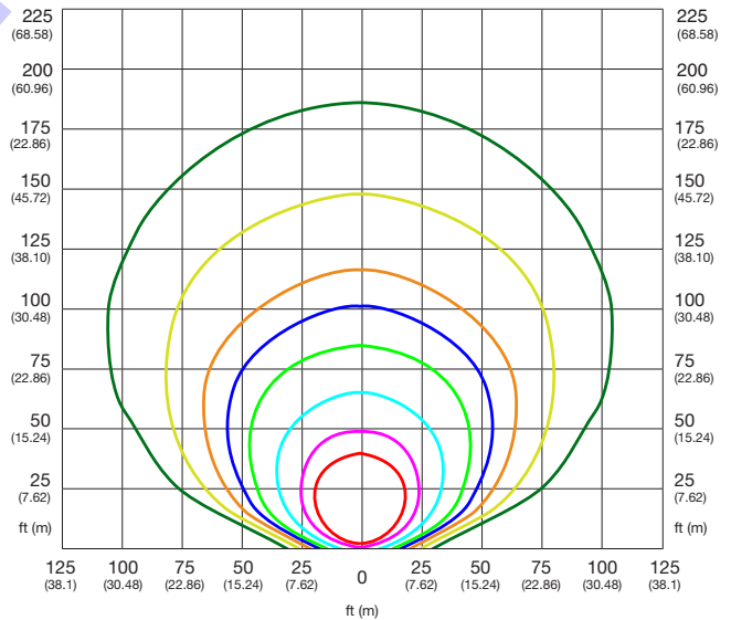
MLT6 METAL HALIDE COVERAGE (4) 1,110W Metal Halide Fixtures
