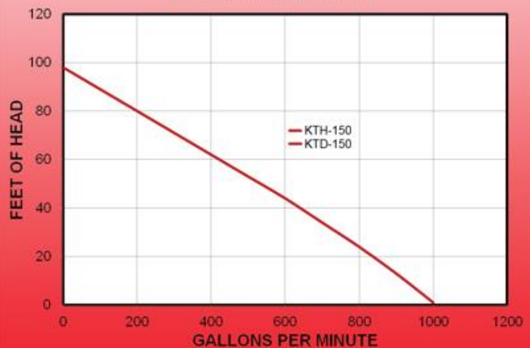
PERFORMANCE CURVE
