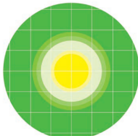
Light plot - GB8LED
