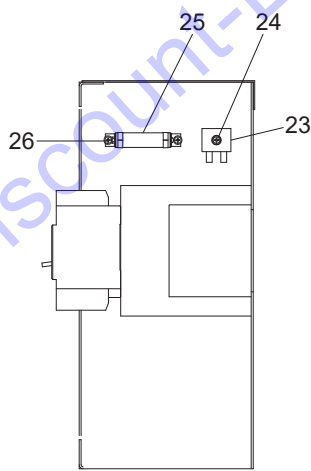
VIEW - A
