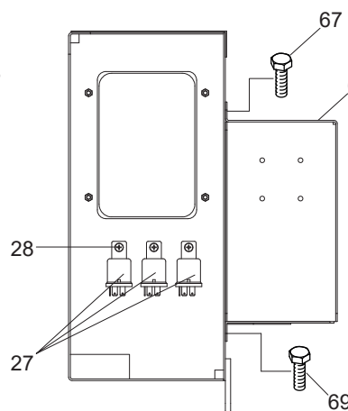
VIEW-B
