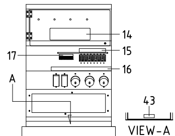
TERMINAL PLATE
