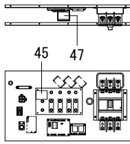
SWITCH BOARD
