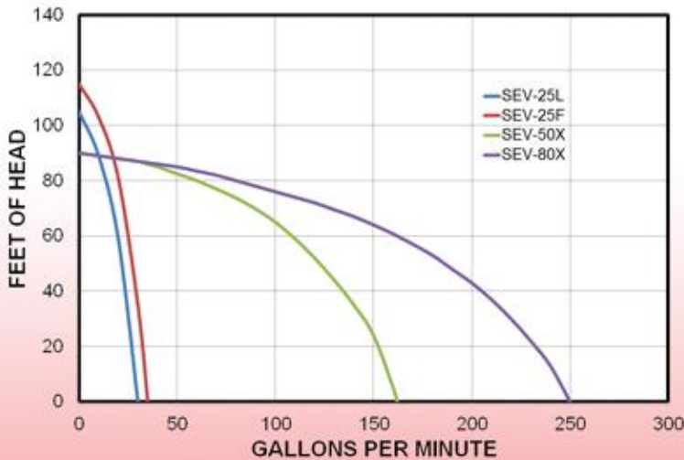
PERFORMANCE CURVES
