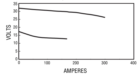
VOLT/AMP CURVES
