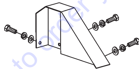
Figure 6. V-Belt Cover
