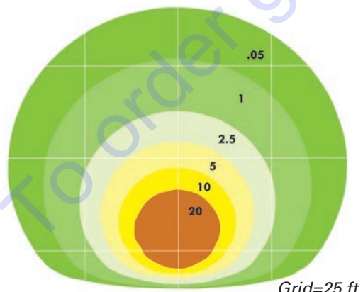
Light Plot
