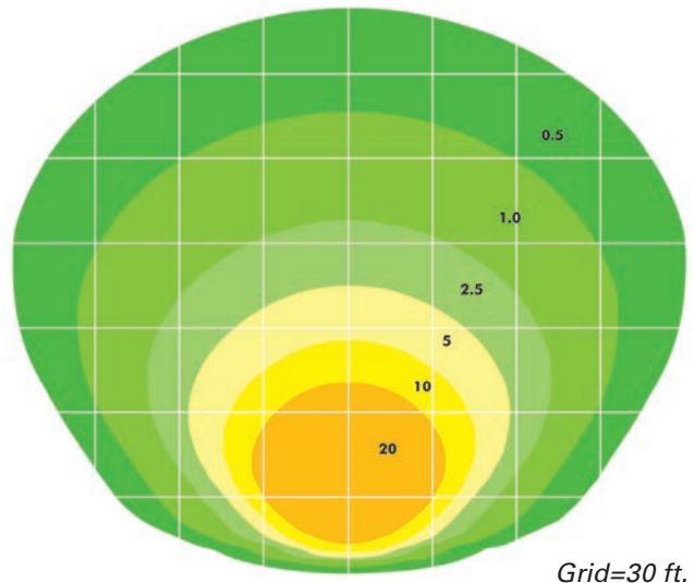
Light Plot
