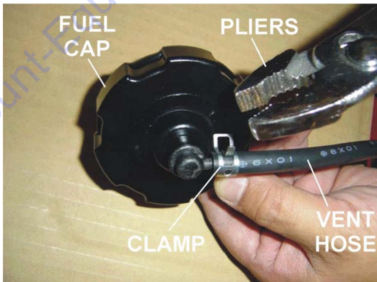
Figure 1. Fuel Cap Removal
