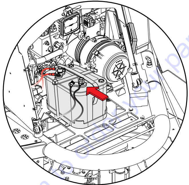
Figure 2. Battery Disconnection
