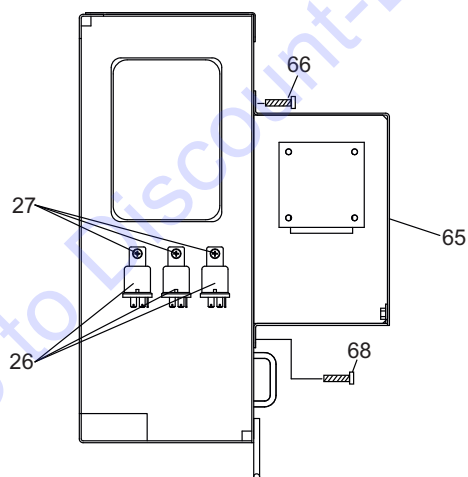
VIEW-B
