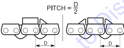
Diamond chain pitch
