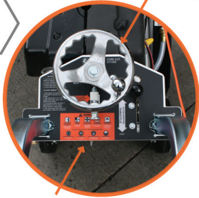
Heavy Duty Adjustable Handles and Precision Screw Feed Raise and Lower System
