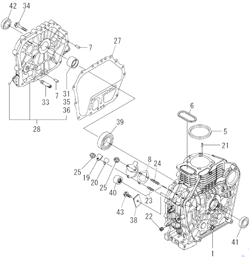
2-06598018 Abb.1. ZYLINDERBLOCK
