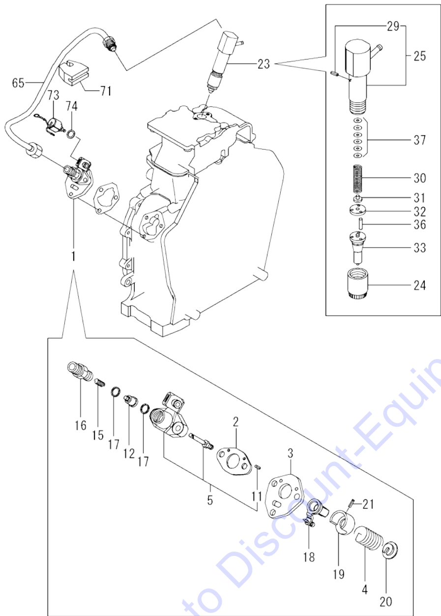
2-06598018 Fig.16. F.I.PUMP & F.I.VALVE
