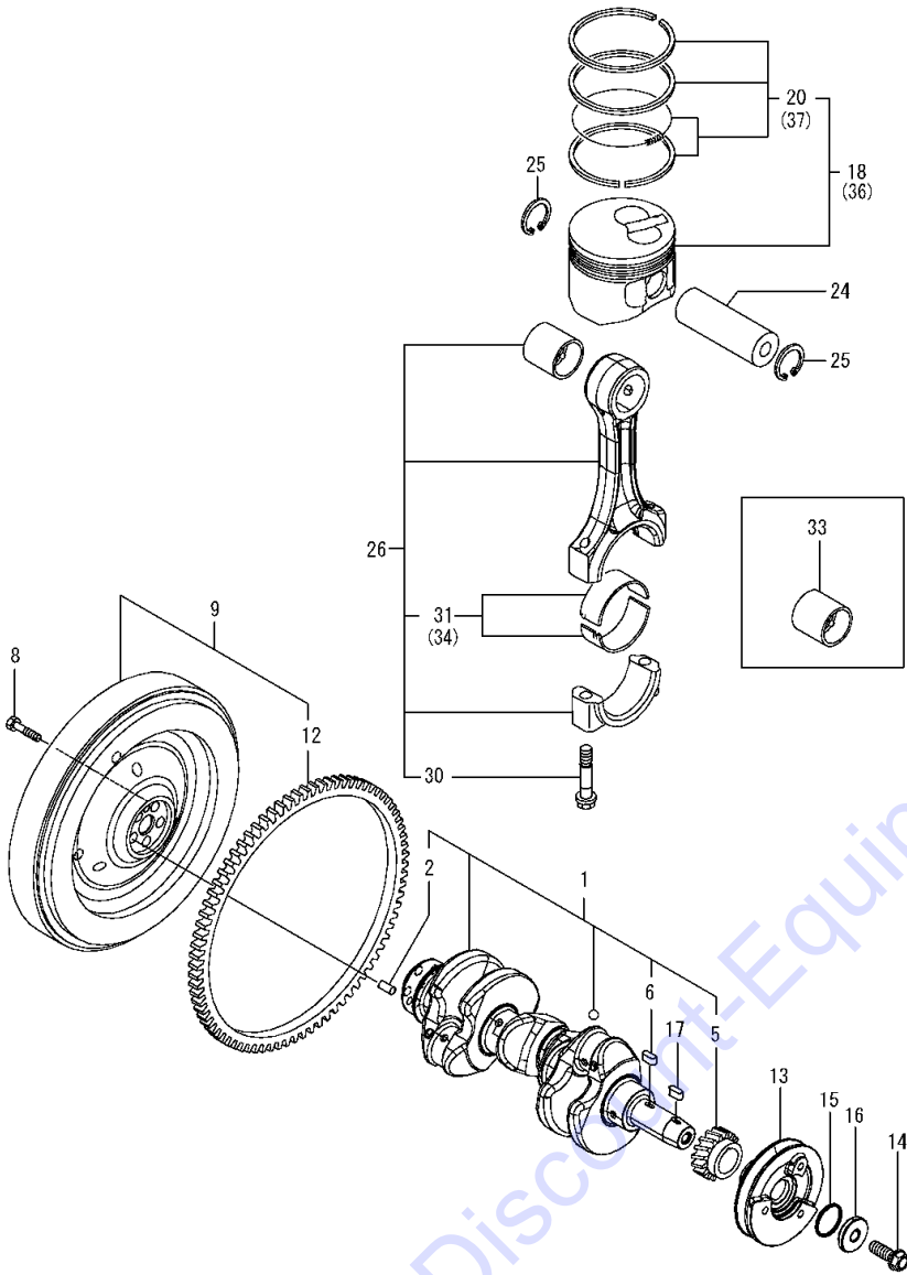
Fig.7. CRANKSHAFT & PISTON
