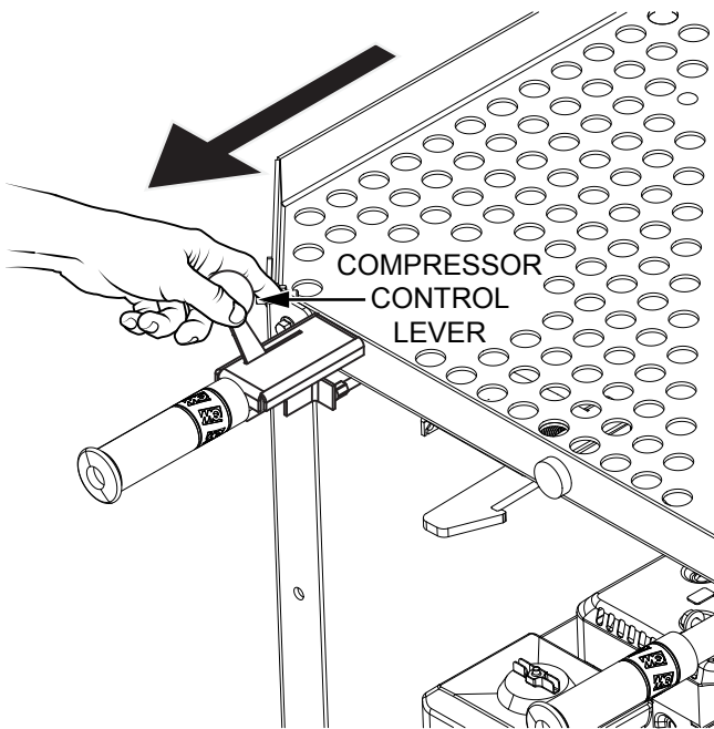
Figure 40. Disengage Compressor
