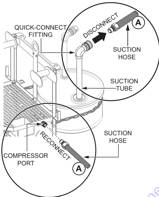
Figure 37. Compressor Connection
