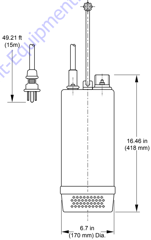
Figure 1. ST2010 Series Dimensions
