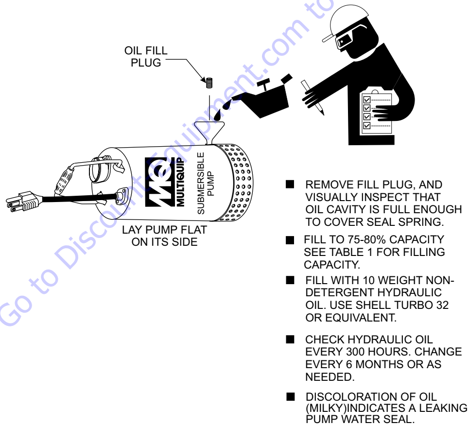
Figure 12. Checking Hydraulic Oil
