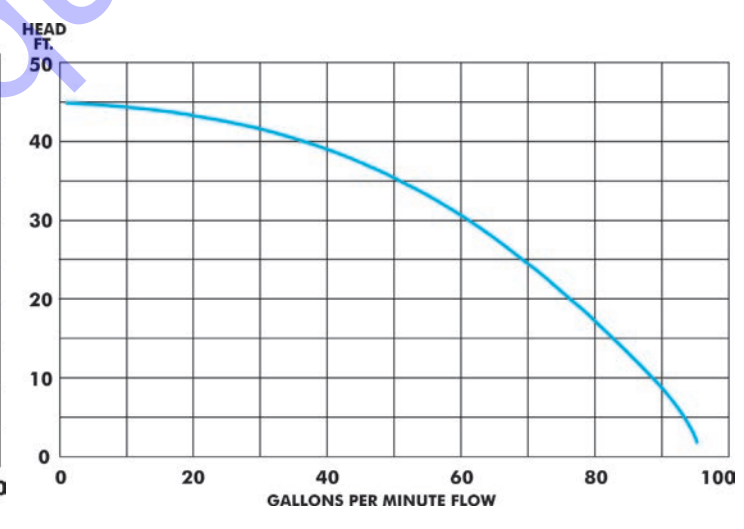
ST2010TCUL Performance Curve 2" Discharge
