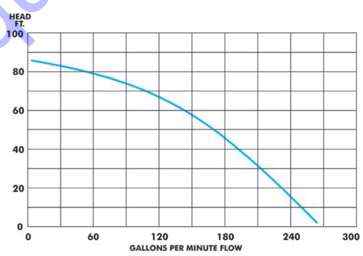
ST3050D Performance Curve 3" Discharge
