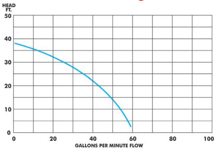
ST2038P Performance Curve 2" Discharge
