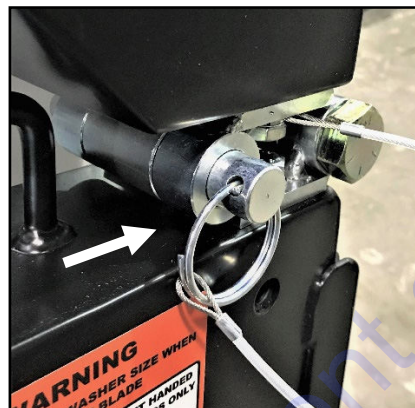
Detent Pin with Guard Fully Upward
