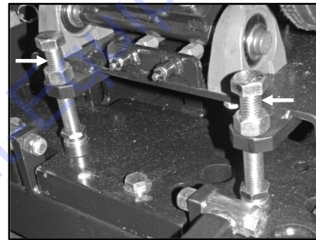
Belt Tension Bolt
