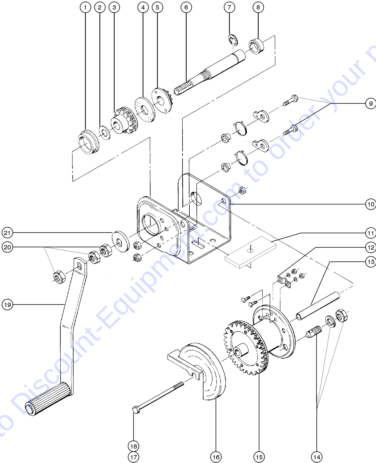
Figure 204.1 Winch Components
