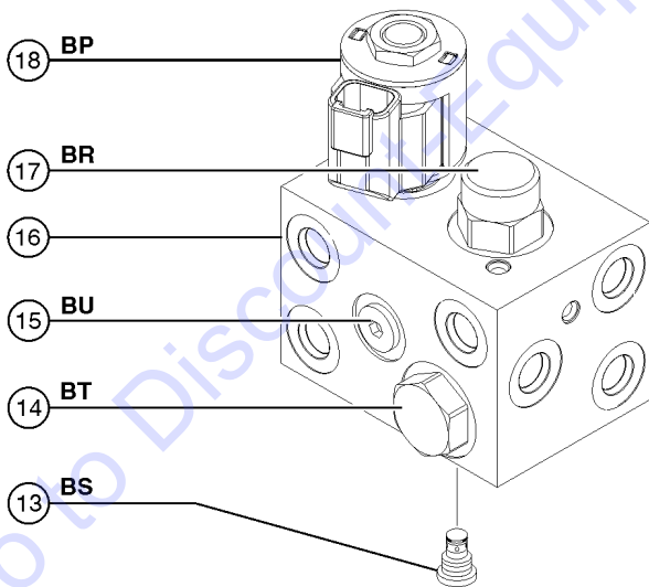
Jib Manifold
