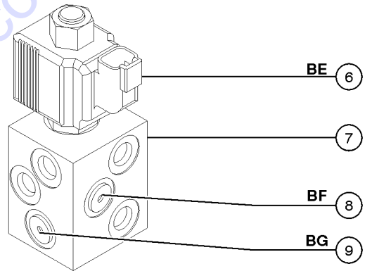
Jib Manifold
