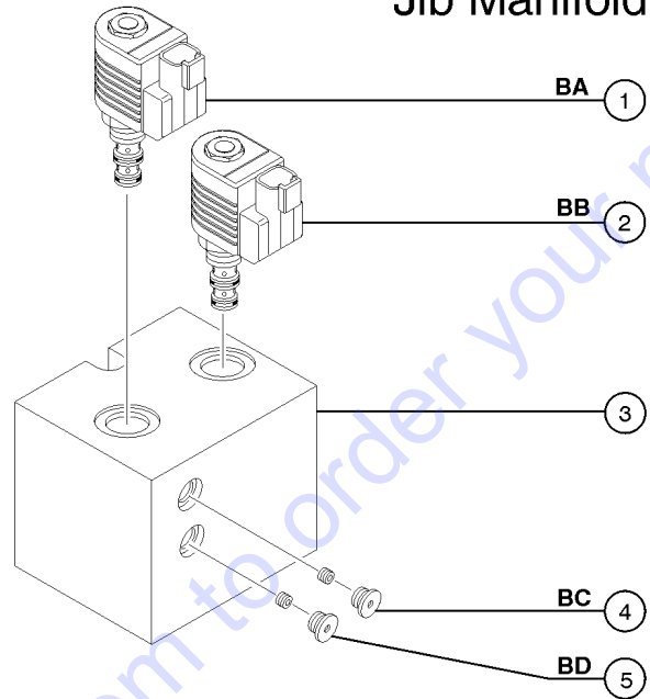
Jib Manifold
