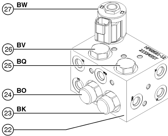
Jib Manifold
