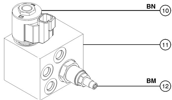
Jib Manifold
