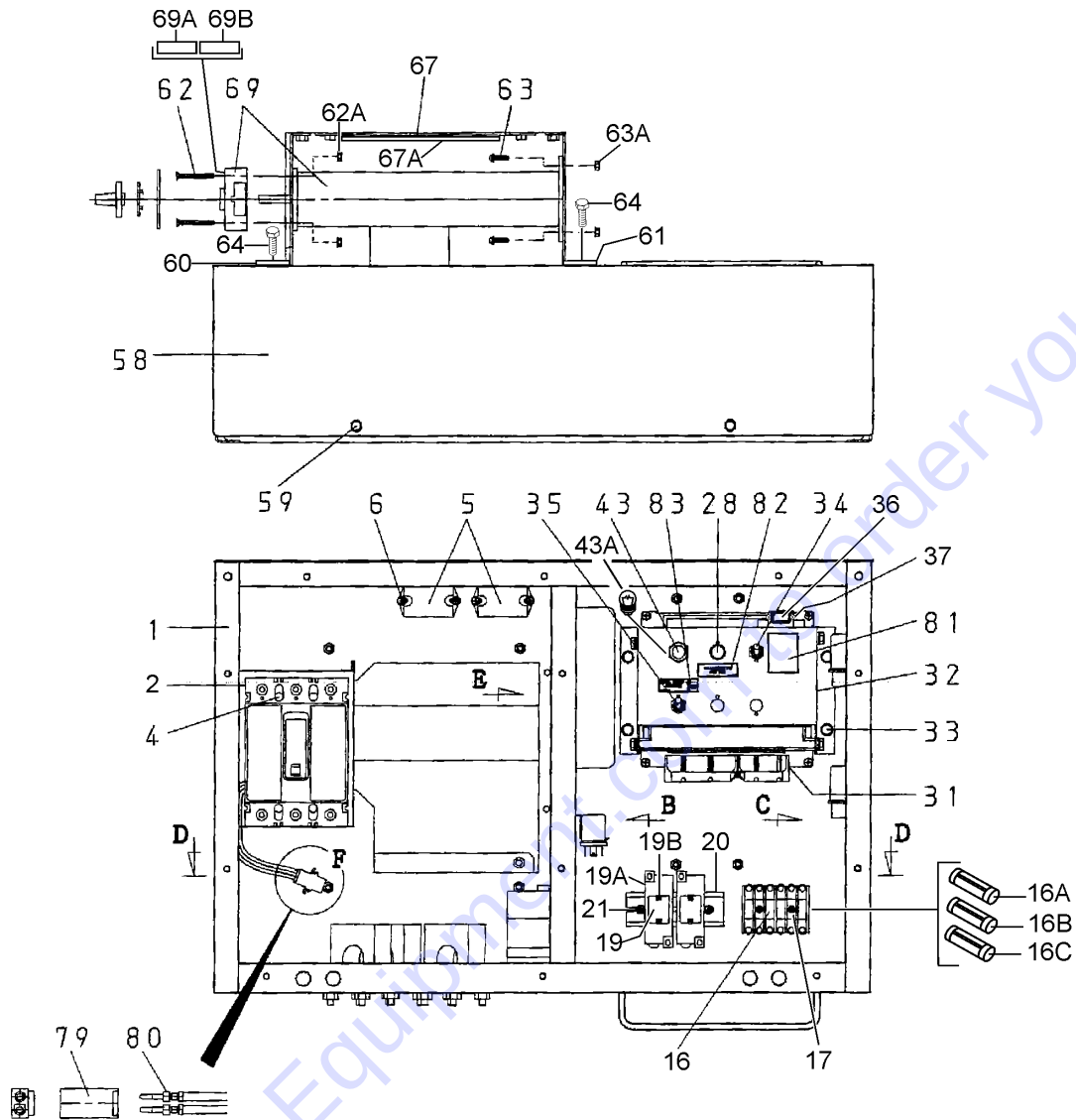
DETAIL-F
