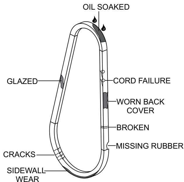
Figure 57. V-Belt Inspection
