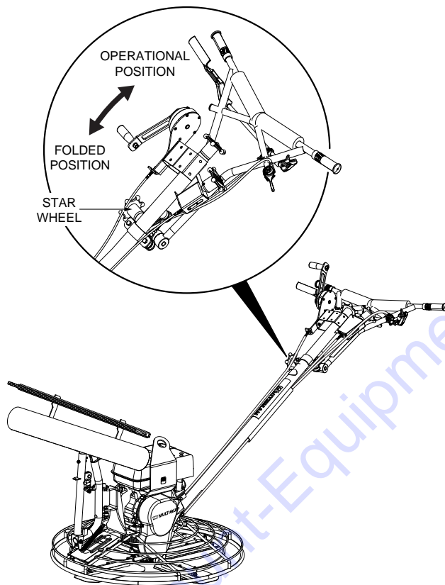
Figure 5. Handlebar (Operational Position)
