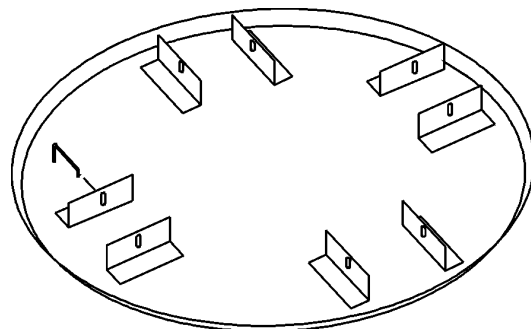
Figure 52. Float Disc/Pan
