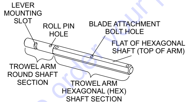
Figure 66. Trowel Arm
