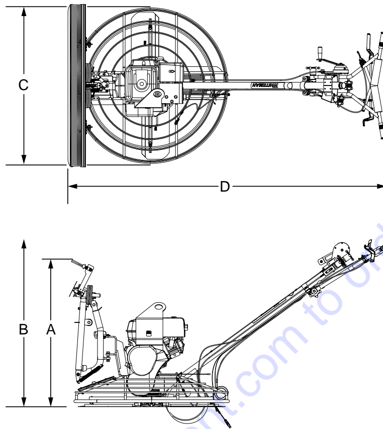
Figure 1. Dimensions
