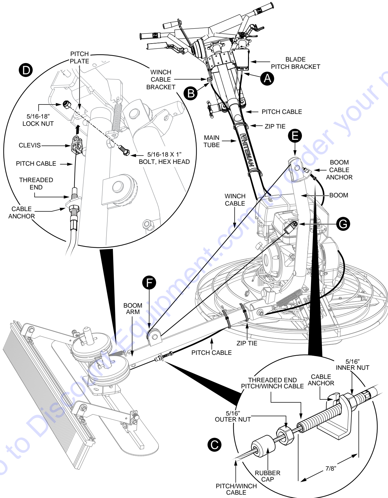
Figure 28. Fresno Pitch/Winch Cable Installation
