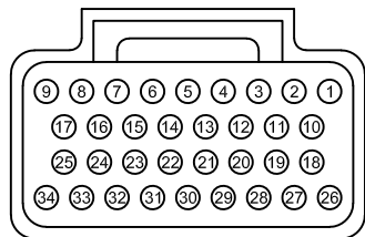
J1 CONNECTOR
